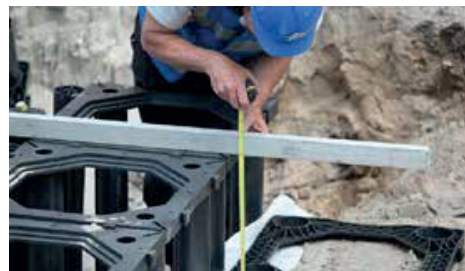
Measure the needed height.
